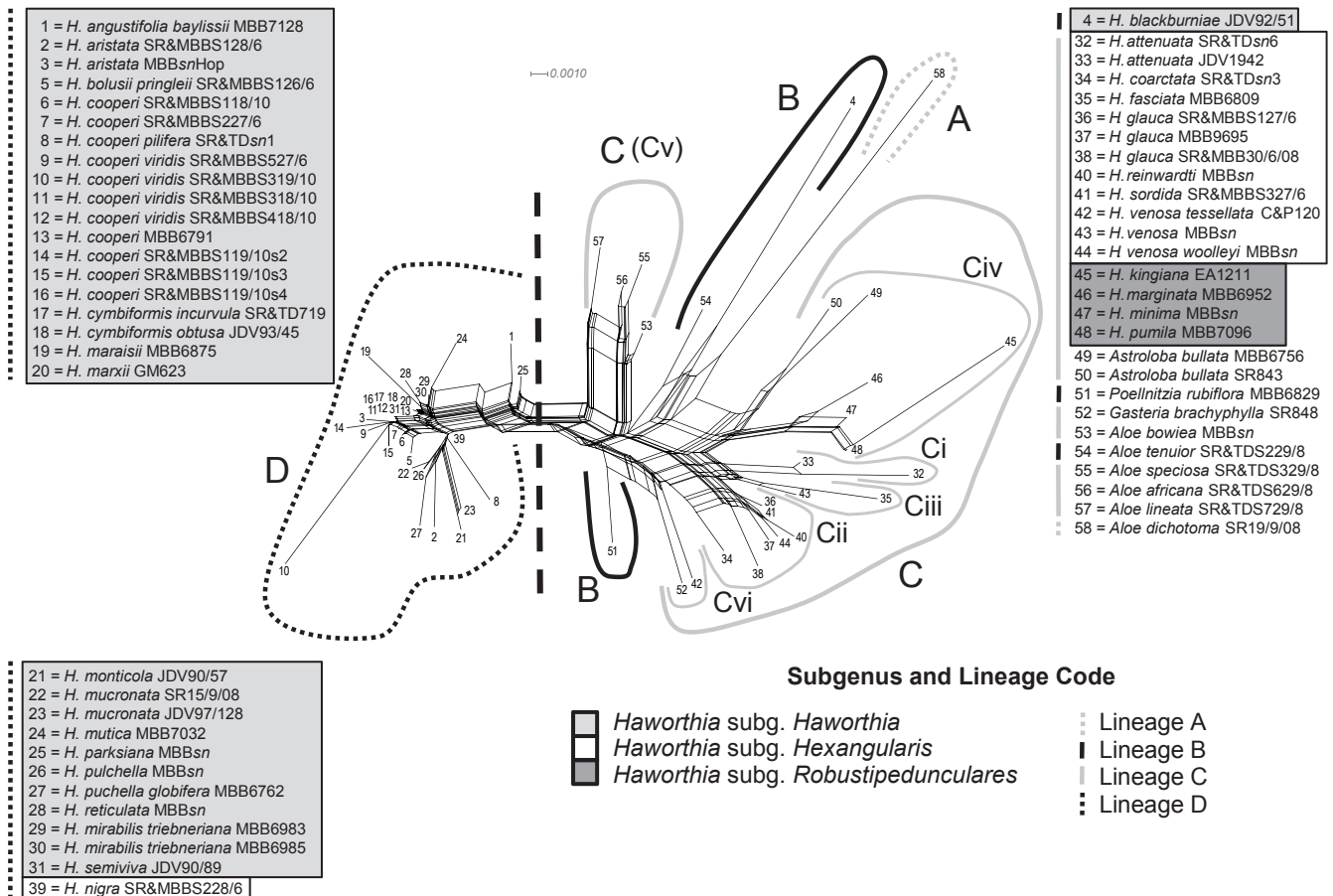
Fig. 3. Splits graph for chloroplast DNA (cpDNA) sequences of Alooideae. Two major branches were recovered (i.e., lineage D and other lineages [A–C]). The major lineages recovered are more or less congruent with the major cpDNA lineages (see Fig. 2a).
